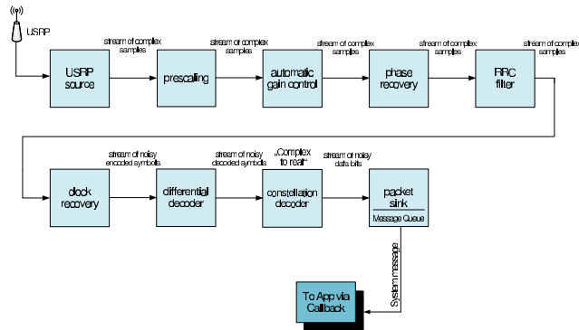
Fig. 2. Flow graph of the receiver.
