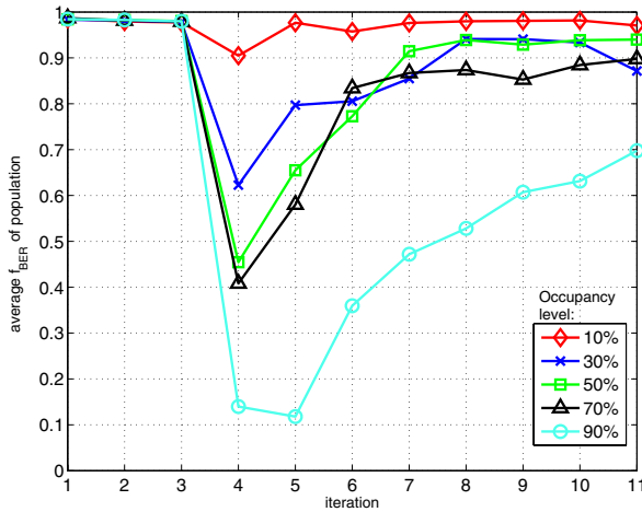
Fig. 4. Channel adaptation for several spectrum occupancy levels. Convergence behavior of f_{min\_BER} (1) as a function of the number of iterations.
