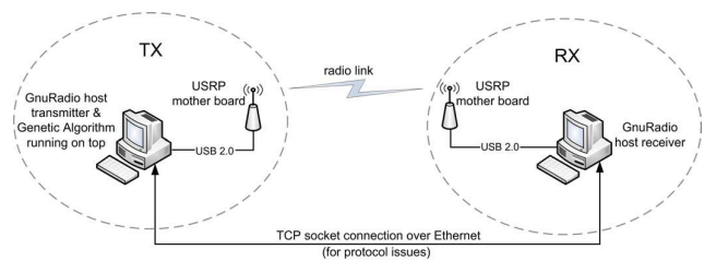
Fig. 1. Testing setup of a Cognitive Radio.
