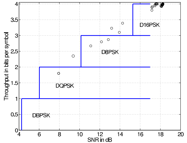
Fig. 3. Weight determination as a function of the transmission SNR in order to achieve optimal rate.
