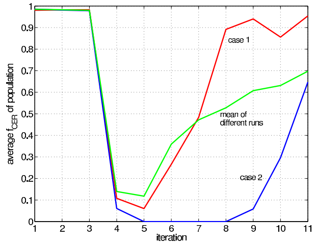
Fig. 5. Convergence analysis for the scenario where 90% of the channels are jammed.
